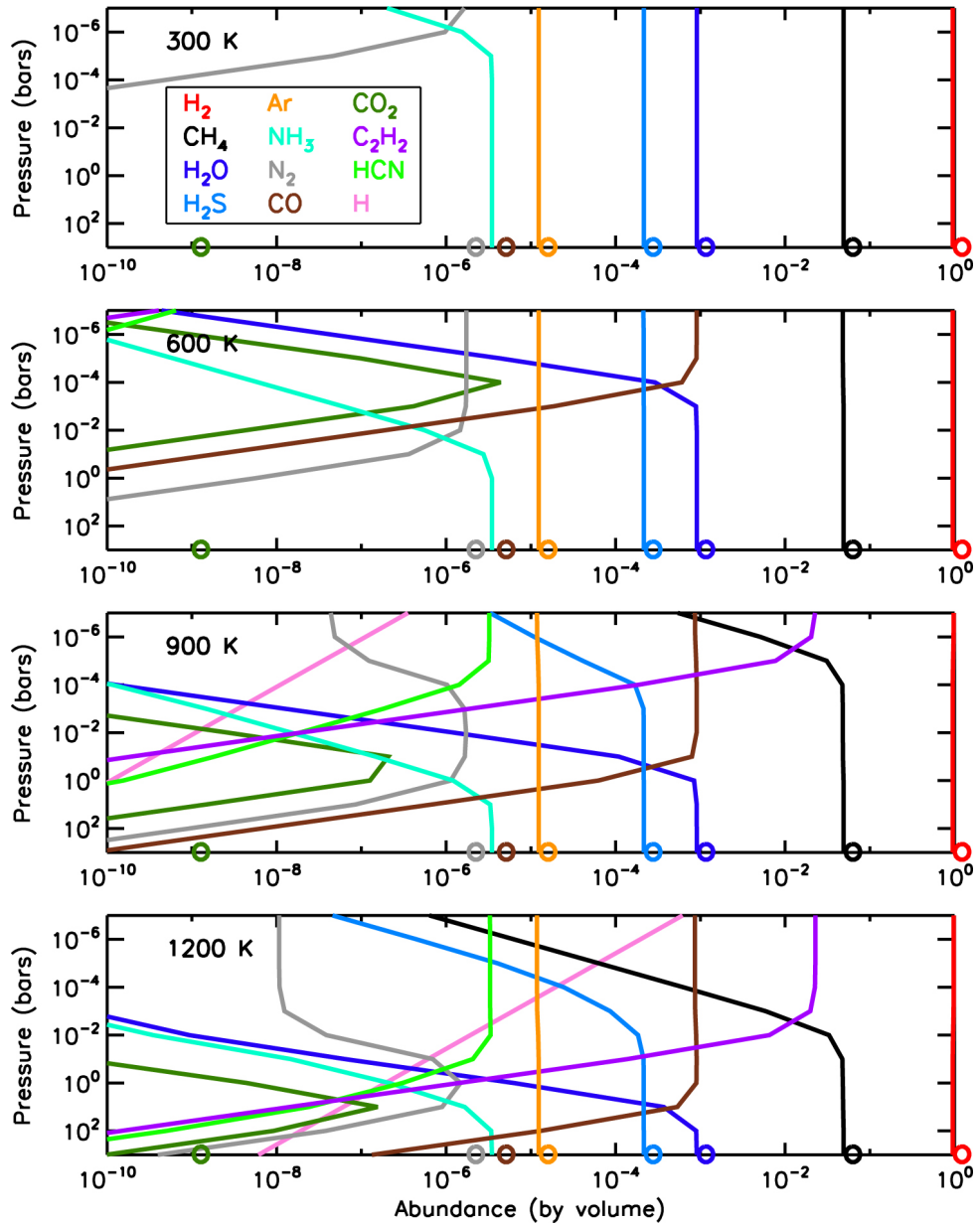
Figure 5. from Edwin A. Bergin et al 2023 Astrophys. J. Lett. 949 doi:10.3847/2041-8213/acd377 https://dx.doi.org/10.3847/2041-8213/acd377 © 2023. The Author(s). Published by the American Astronomical Society.
