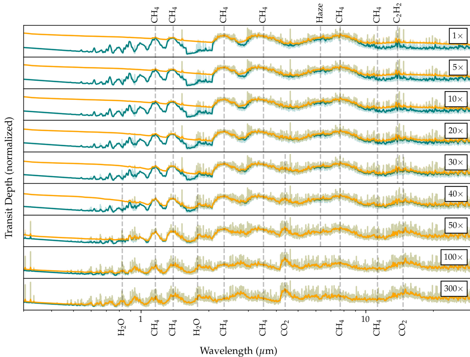
Figure 4. from Edwin A. Bergin et al 2023 Astrophys. J. Lett. 949 doi:10.3847/2041-8213/acd377 https://dx.doi.org/10.3847/2041-8213/acd377 © 2023. The Author(s). Published by the American Astronomical Society.
