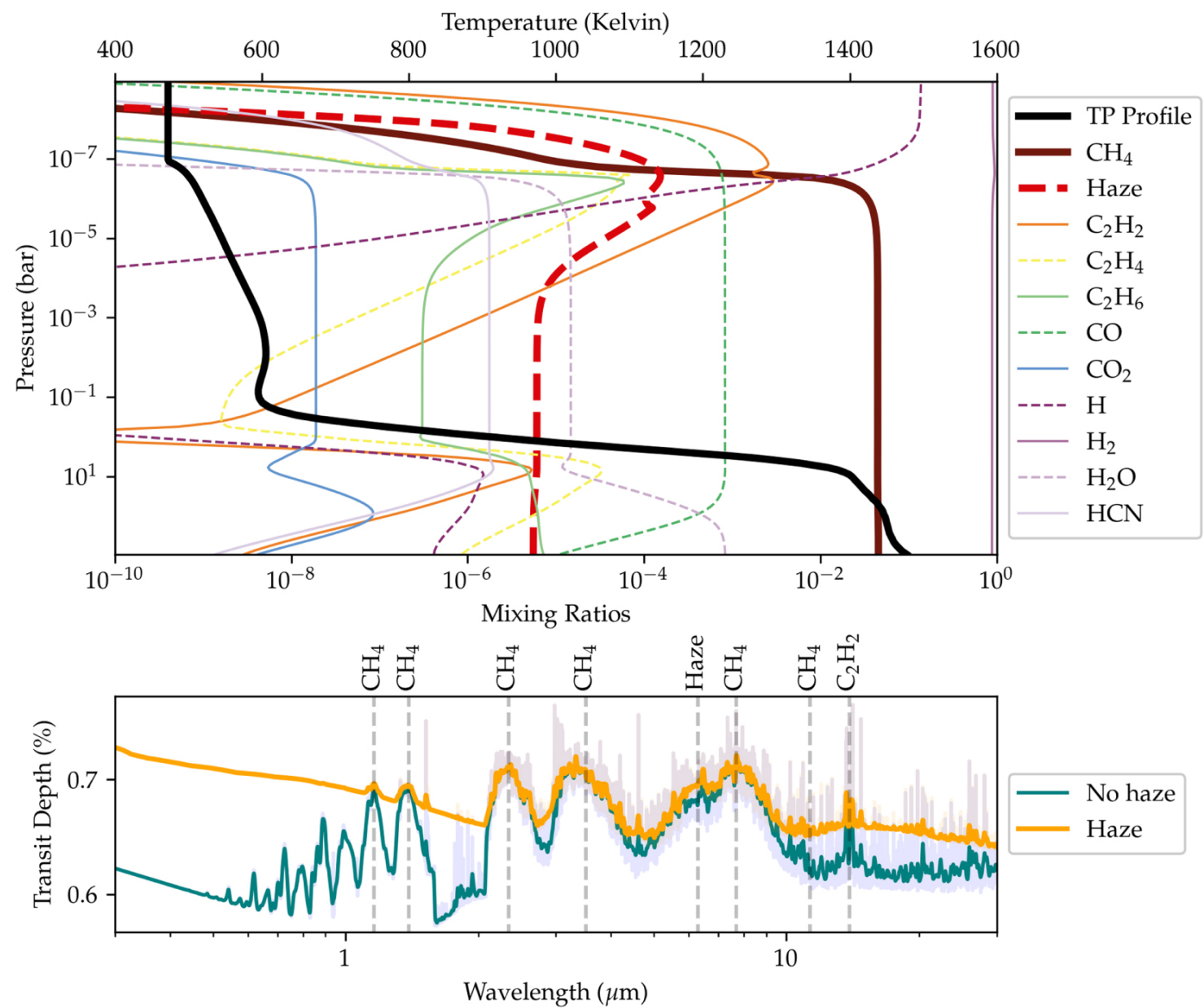
Figure 3. from Edwin A. Bergin et al 2023 Astrophys. J. Lett. 949 doi:10.3847/2041-8213/acd377 https://dx.doi.org/10.3847/2041-8213/acd377 © 2023. The Author(s). Published by the American Astronomical Society.
