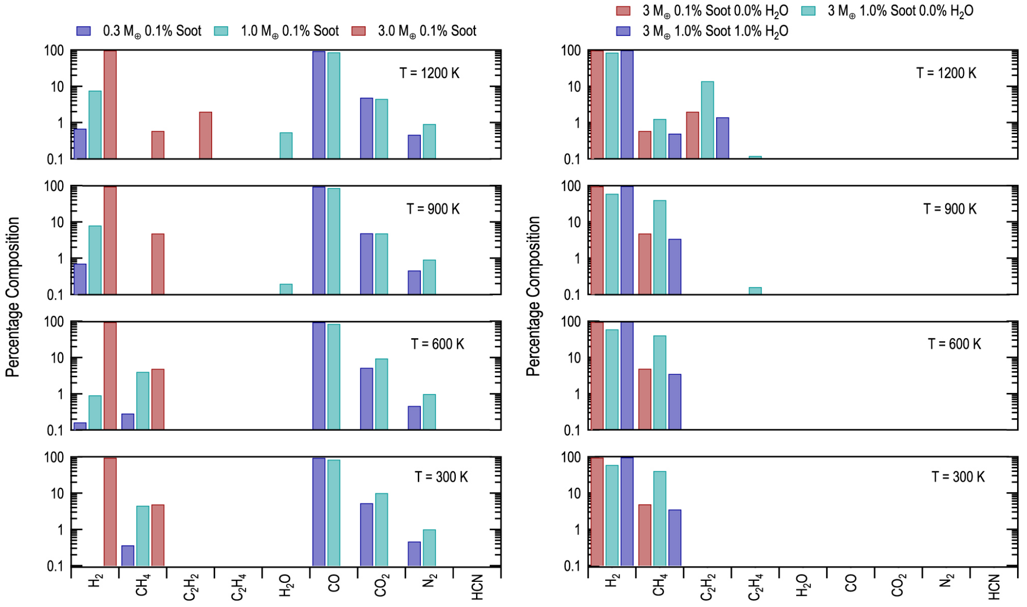
Figure 2. from Edwin A. Bergin et al 2023 Astrophys. J. Lett. 949 doi:10.3847/2041-8213/acd377 https://dx.doi.org/10.3847/2041-8213/acd377 © 2023. The Author(s). Published by the American Astronomical Society.
