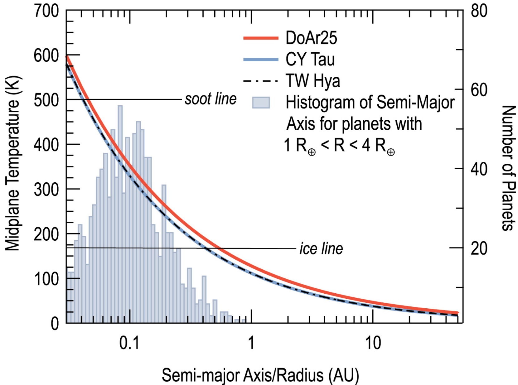
Figure 1. from Edwin A. Bergin et al 2023 Astrophys. J. Lett. 949 doi:10.3847/2041-8213/acd377 https://dx.doi.org/10.3847/2041-8213/acd377 © 2023. The Author(s). Published by the American Astronomical Society.
