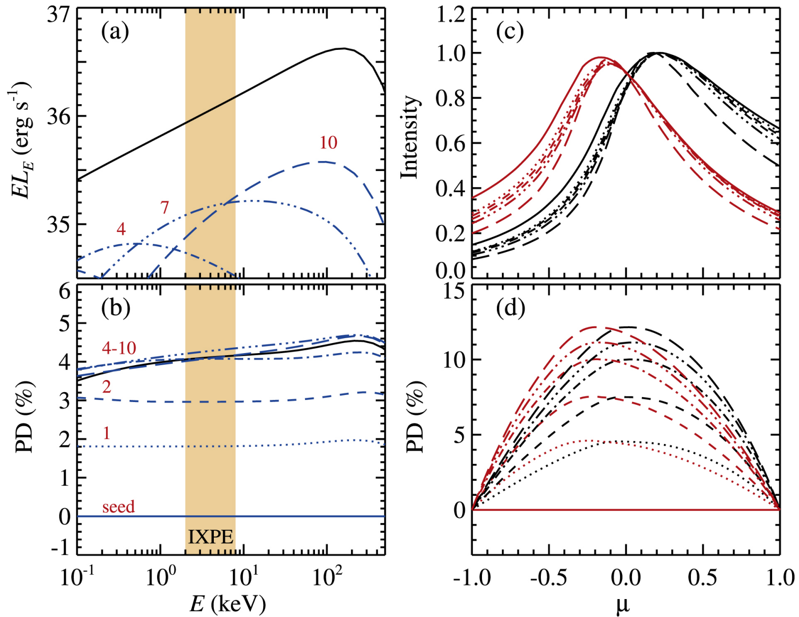
Figure 5. from Juri Poutanen et al 2023 Astrophys. J. Lett. 949 doi:10.3847/2041-8213/acd33e https://dx.doi.org/10.3847/2041-8213/acd33e © 2023. The Author(s). Published by the American Astronomical Society.
