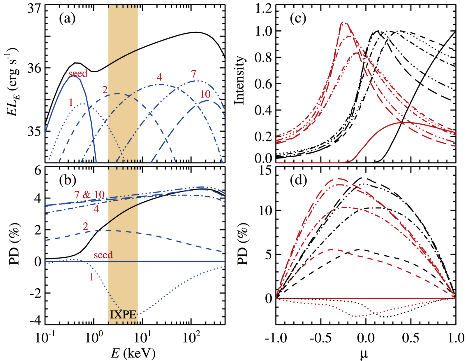
Figure 4. from Juri Poutanen et al 2023 Astrophys. J. Lett. 949 doi:10.3847/2041-8213/acd33e https://dx.doi.org/10.3847/2041-8213/acd33e © 2023. The Author(s). Published by the American Astronomical Society.
