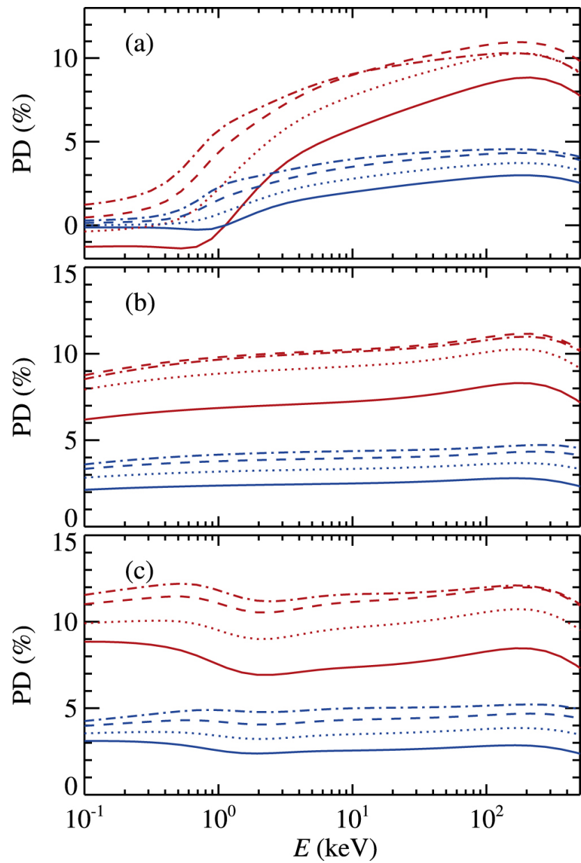
Figure 3. from Juri Poutanen et al 2023 Astrophys. J. Lett. 949 doi:10.3847/2041-8213/acd33e https://dx.doi.org/10.3847/2041-8213/acd33e © 2023. The Author(s). Published by the American Astronomical Society.
