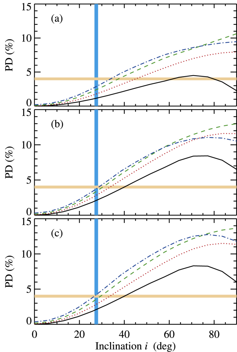
Figure 2. from Juri Poutanen et al 2023 Astrophys. J. Lett. 949 doi:10.3847/2041-8213/acd33e https://dx.doi.org/10.3847/2041-8213/acd33e © 2023. The Author(s). Published by the American Astronomical Society.
