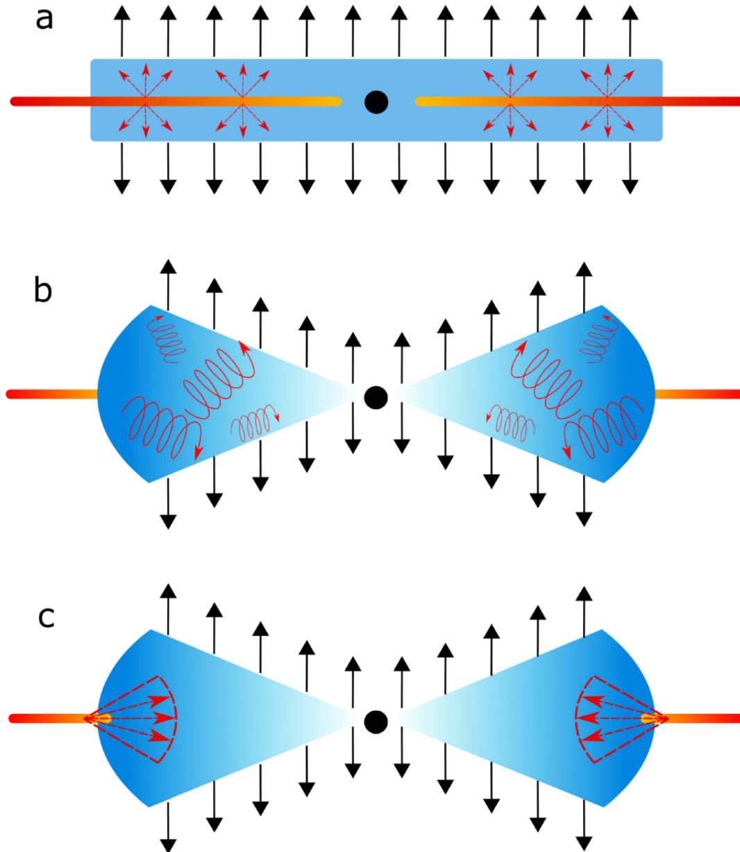
Figure 1. from Juri Poutanen et al 2023 Astrophys. J. Lett. 949 doi:10.3847/2041-8213/acd33e https://dx.doi.org/10.3847/2041-8213/acd33e © 2023. The Author(s). Published by the American Astronomical Society.
