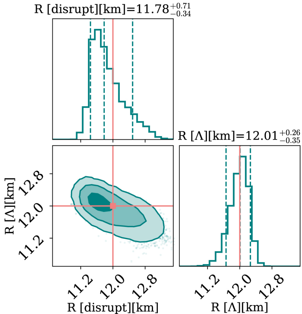
Figure 5. from Teagan A. Clarke et al 2023 Astrophys. J. Lett. 949 doi:10.3847/2041-8213/acd33b https://dx.doi.org/10.3847/2041-8213/acd33b © 2023. The Author(s). Published by the American Astronomical Society.
