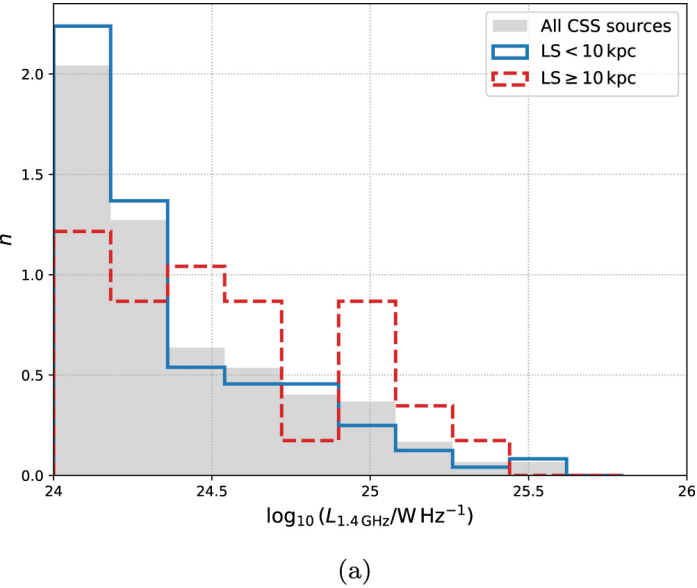
Figure 5. from Yjan A. Gordon et al 2023 Astrophys. J. Lett. 948 doi:10.3847/2041-8213/accf0a https://dx.doi.org/10.3847/2041-8213/accf0a © 2023. The Author(s). Published by the American Astronomical Society.
