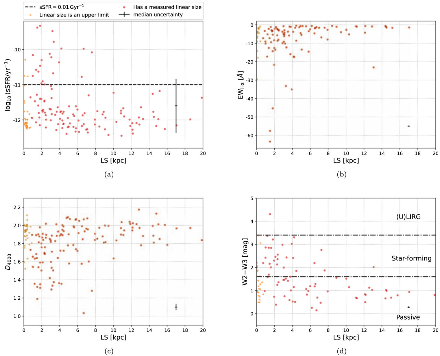
Figure 3. from Yjan A. Gordon et al 2023 Astrophys. J. Lett. 948 doi:10.3847/2041-8213/accf0a https://dx.doi.org/10.3847/2041-8213/accf0a © 2023. The Author(s). Published by the American Astronomical Society.
