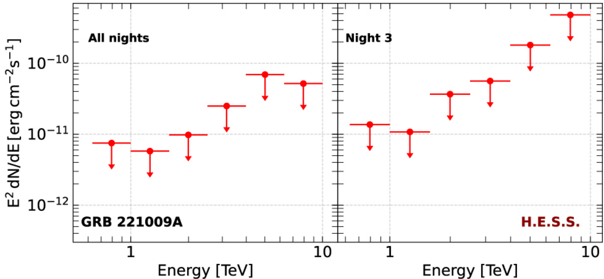
Figure 2. from F. Aharonian et al 2023 Astrophys. J. Lett. 946 doi:10.3847/2041-8213/acc405 https://dx.doi.org/10.3847/2041-8213/acc405 © 2023. The Author(s). Published by the American Astronomical Society.
