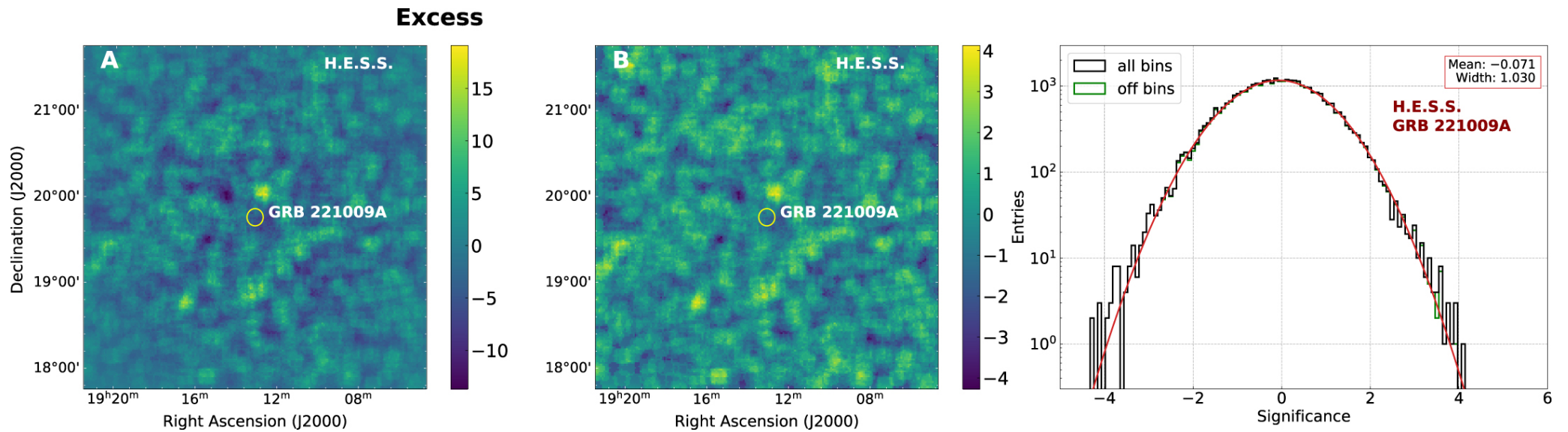
Figure 1. from F. Aharonian et al 2023 Astrophys. J. Lett. 946 doi:10.3847/2041-8213/acc405 https://dx.doi.org/10.3847/2041-8213/acc405 © 2023. The Author(s). Published by the American Astronomical Society.
