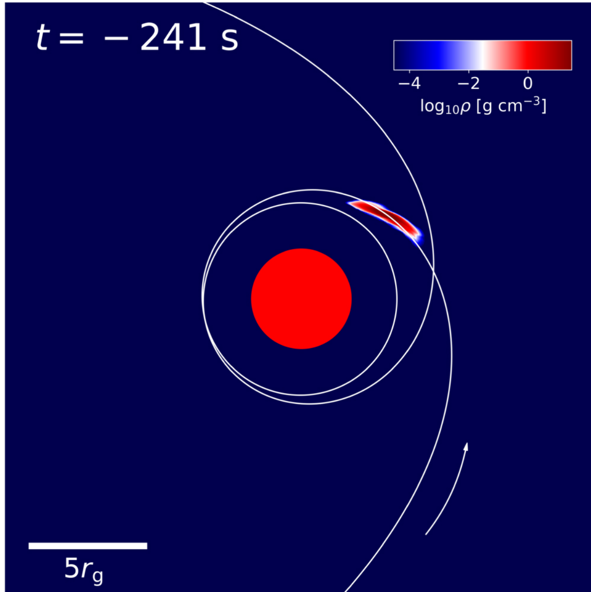
Figure 2. from Taeho Ryu et al 2023 Astrophys. J. Lett. 946 doi:10.3847/2041-8213/acc390 https://dx.doi.org/10.3847/2041-8213/acc390 © 2023. The Author(s). Published by the American Astronomical Society.
