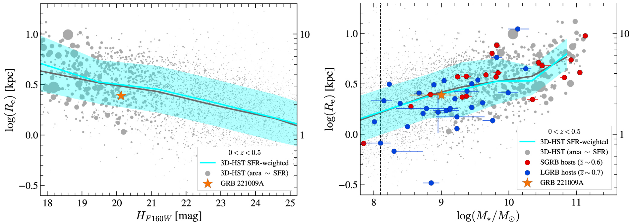
Figure 8. from A. J. Levan et al 2023 Astrophys. J. Lett. 946 doi:10.3847/2041-8213/acc2c1 https://dx.doi.org/10.3847/2041-8213/acc2c1 © 2023. The Author(s). Published by the American Astronomical Society.
