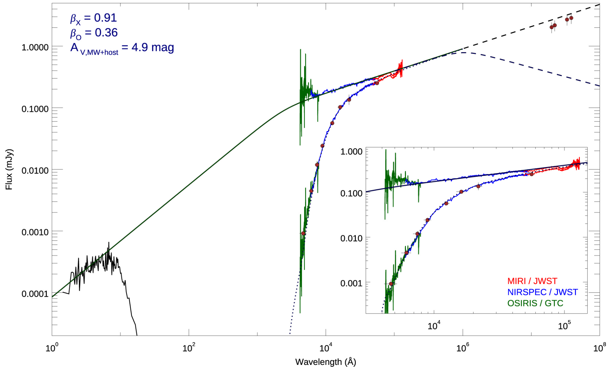
Figure 7. from A. J. Levan et al 2023 Astrophys. J. Lett. 946 doi:10.3847/2041-8213/acc2c1 https://dx.doi.org/10.3847/2041-8213/acc2c1 © 2023. The Author(s). Published by the American Astronomical Society.
