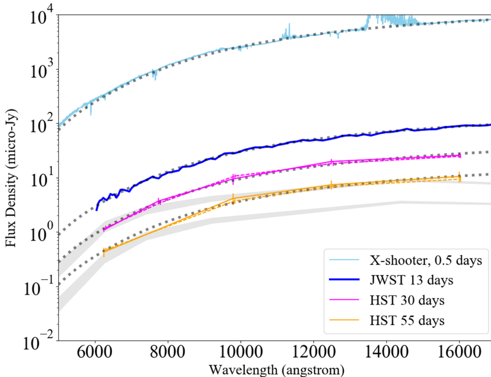
Figure 6. from A. J. Levan et al 2023 Astrophys. J. Lett. 946 doi:10.3847/2041-8213/acc2c1 https://dx.doi.org/10.3847/2041-8213/acc2c1 © 2023. The Author(s). Published by the American Astronomical Society.
