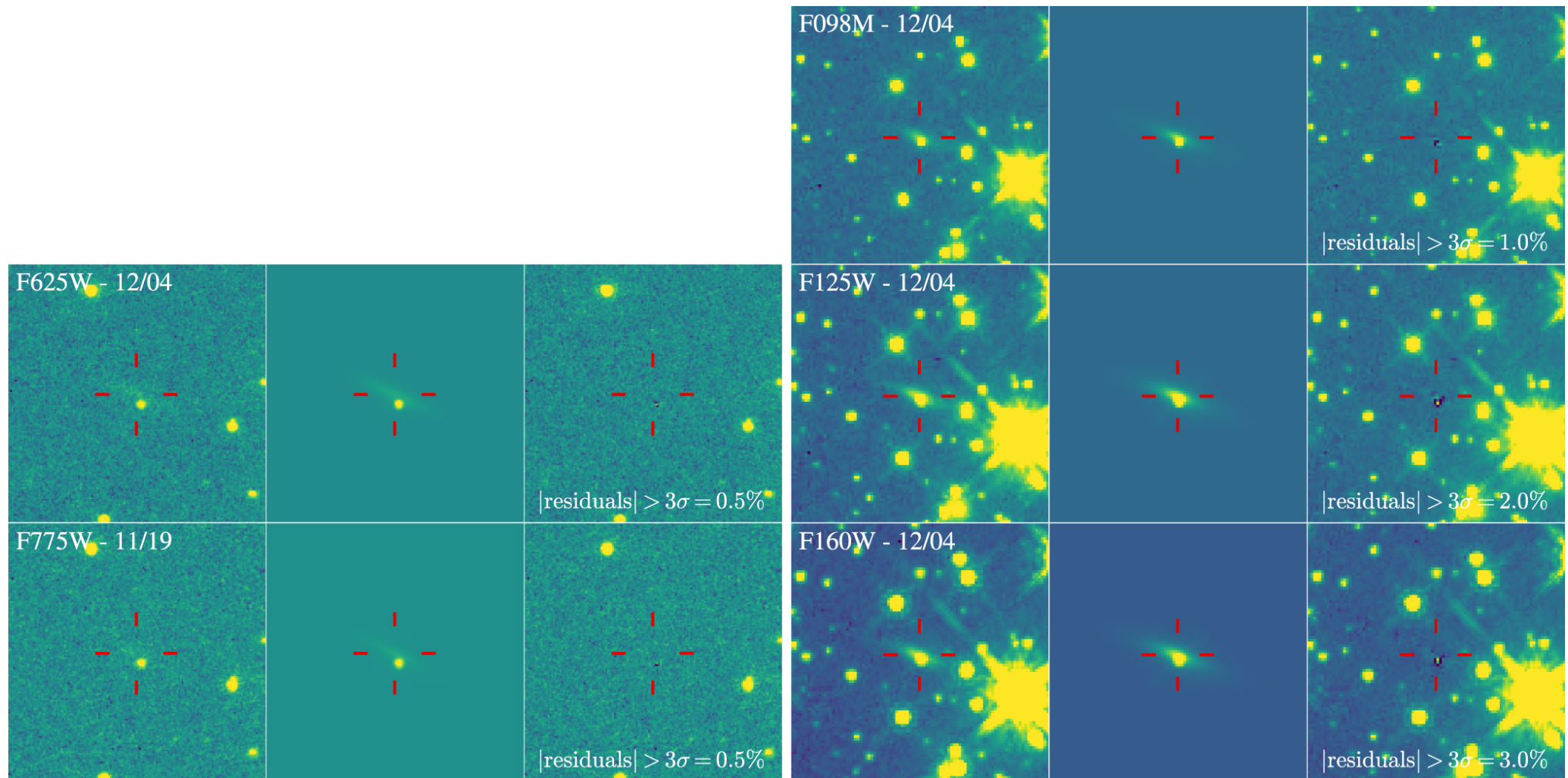
Figure 4. from A. J. Levan et al 2023 Astrophys. J. Lett. 946 doi:10.3847/2041-8213/acc2c1 https://dx.doi.org/10.3847/2041-8213/acc2c1 © 2023. The Author(s). Published by the American Astronomical Society.
