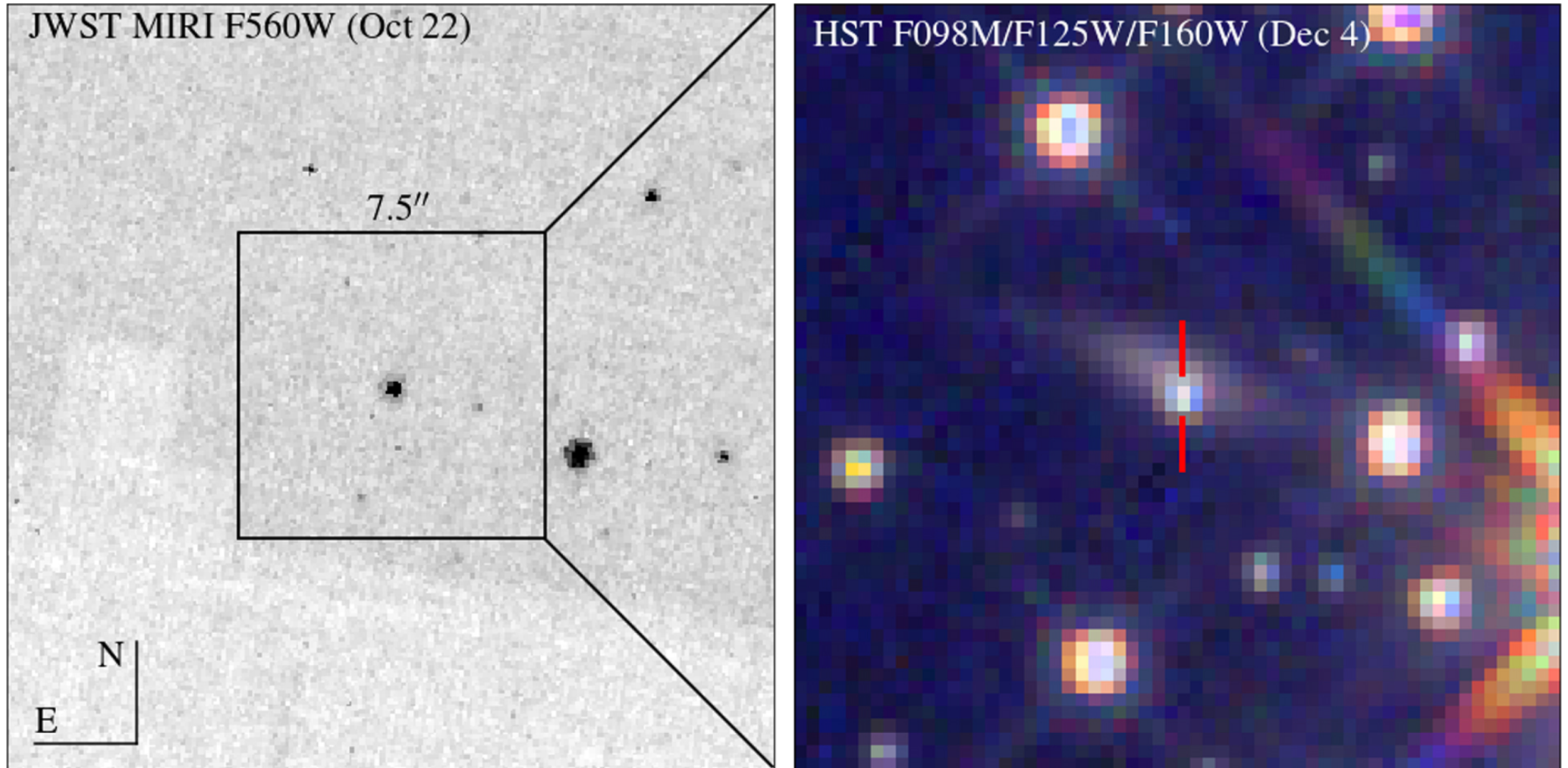
Figure 1. from A. J. Levan et al 2023 Astrophys. J. Lett. 946 doi:10.3847/2041-8213/acc2c1 https://dx.doi.org/10.3847/2041-8213/acc2c1 © 2023. The Author(s). Published by the American Astronomical Society.
