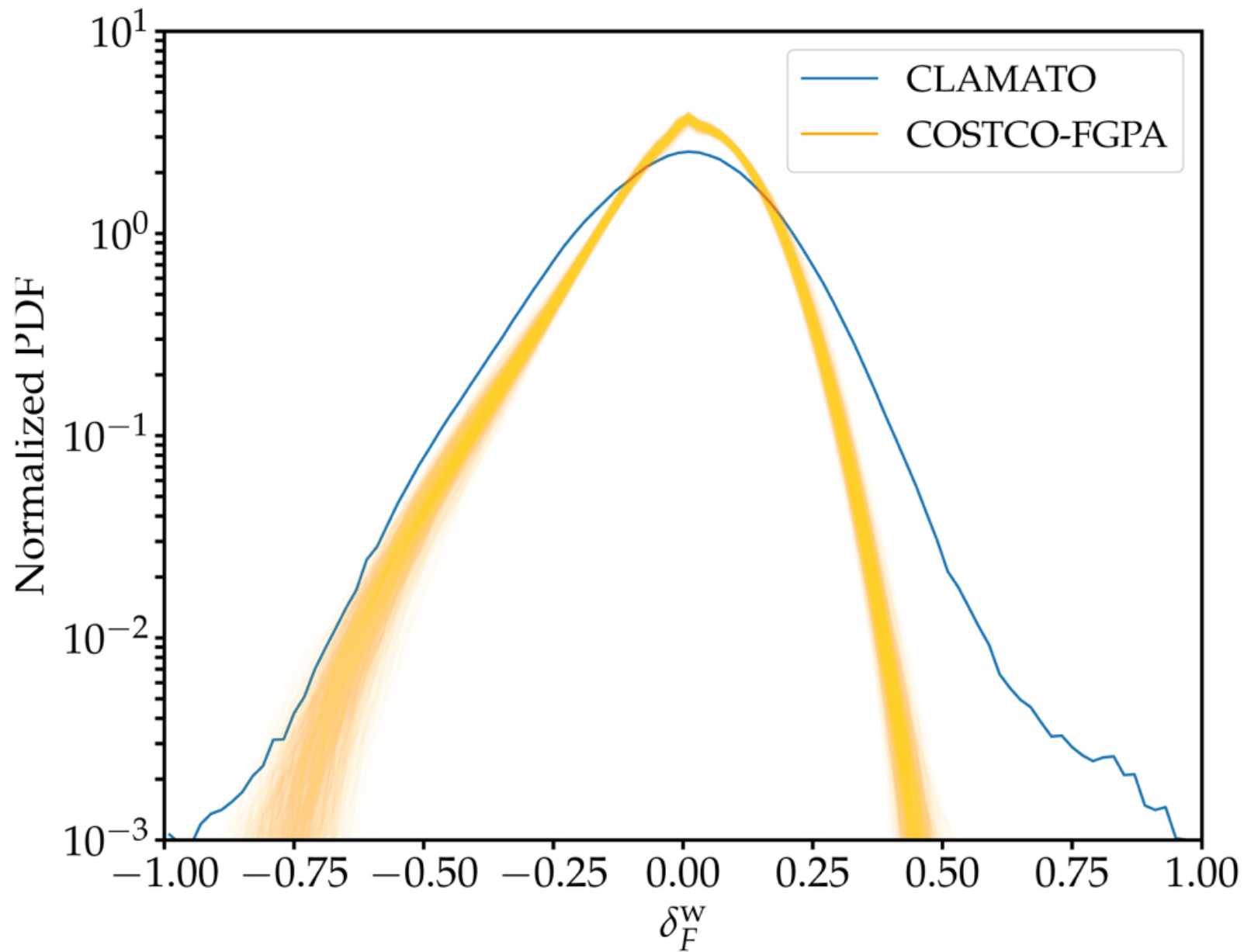
Figure 4. from Chenze Dong et al 2023 Astrophys. J. Lett. 945 doi:10.3847/2041-8213/acba89 https://dx.doi.org/10.3847/2041-8213/acba89 © 2023. The Author(s). Published by the American Astronomical Society.
