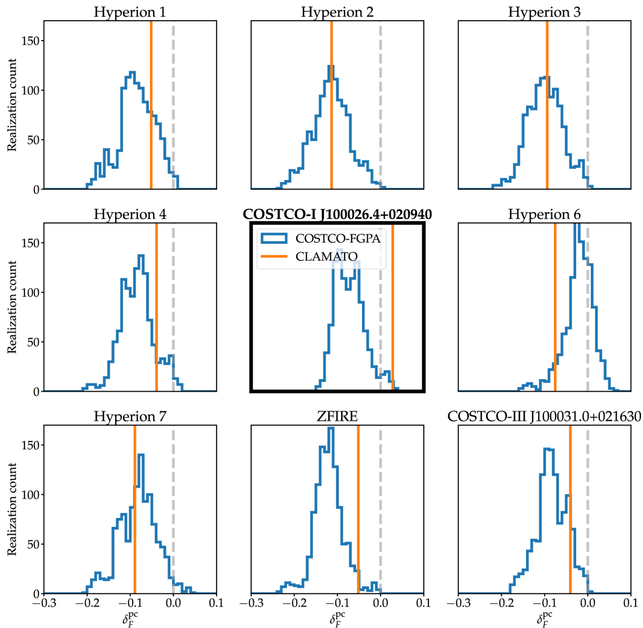
Figure 3. from Chenze Dong et al 2023 Astrophys. J. Lett. 945 doi:10.3847/2041-8213/acba89 https://dx.doi.org/10.3847/2041-8213/acba89 © 2023. The Author(s). Published by the American Astronomical Society.
