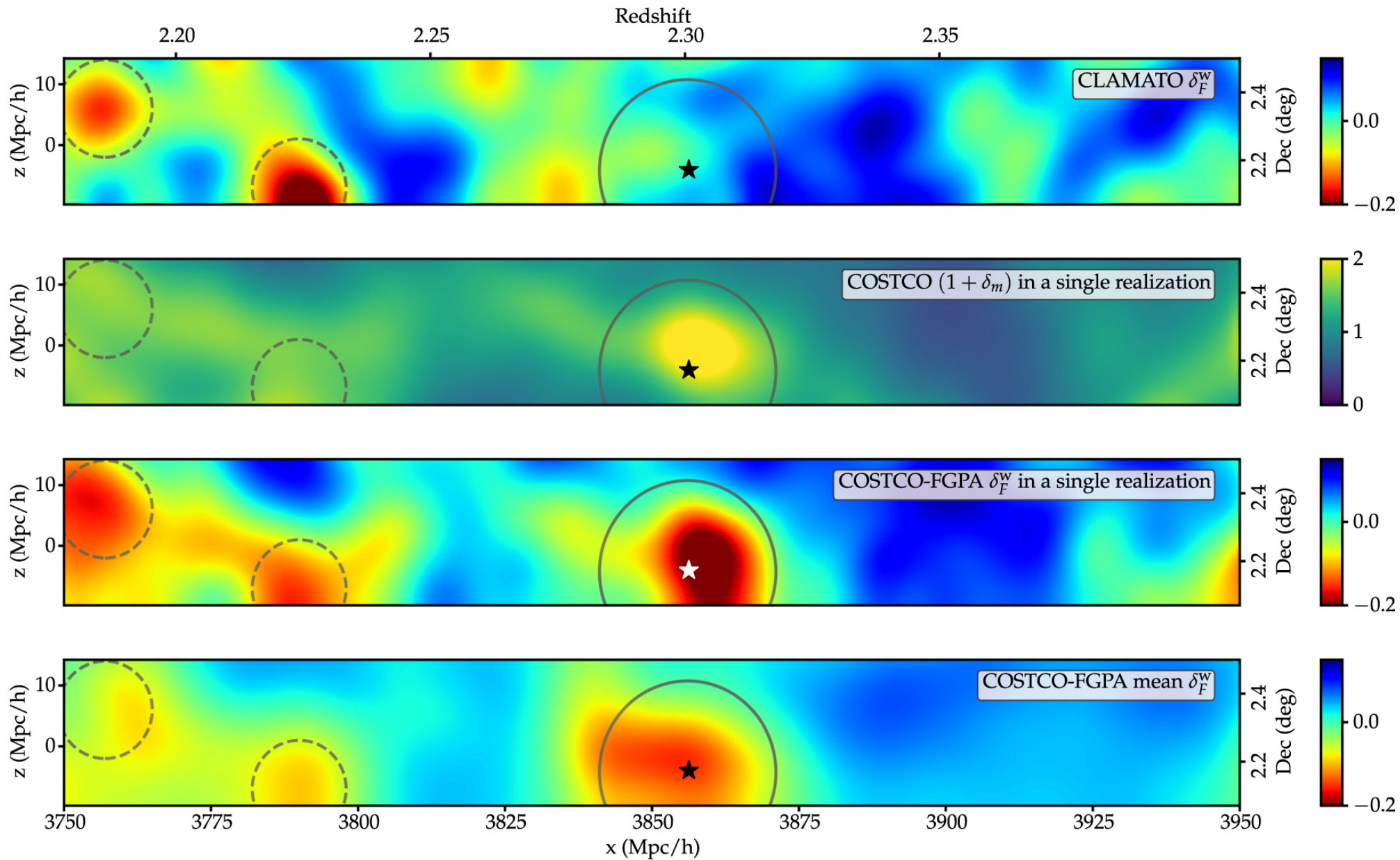
Figure 2. from Chenze Dong et al 2023 Astrophys. J. Lett. 945 doi:10.3847/2041-8213/acba89 https://dx.doi.org/10.3847/2041-8213/acba89 © 2023. The Author(s). Published by the American Astronomical Society.
