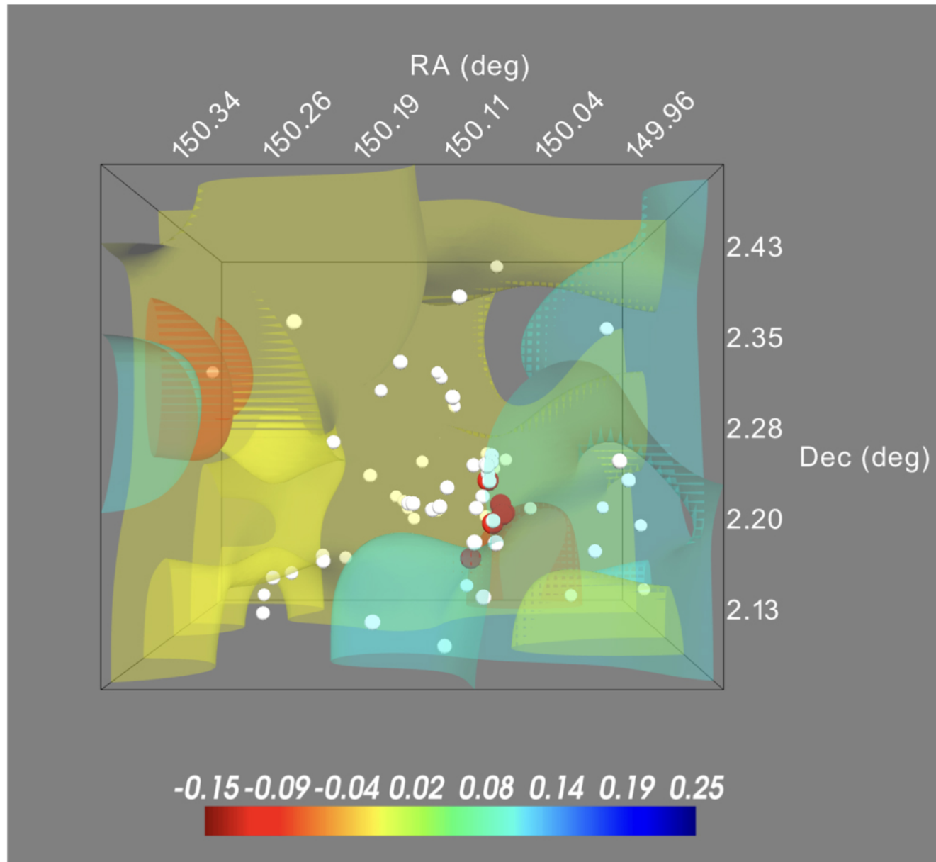
Figure 1. from Chenze Dong et al 2023 Astrophys. J. Lett. 945 doi:10.3847/2041-8213/acba89 https://dx.doi.org/10.3847/2041-8213/acba89 © 2023. The Author(s). Published by the American Astronomical Society.
