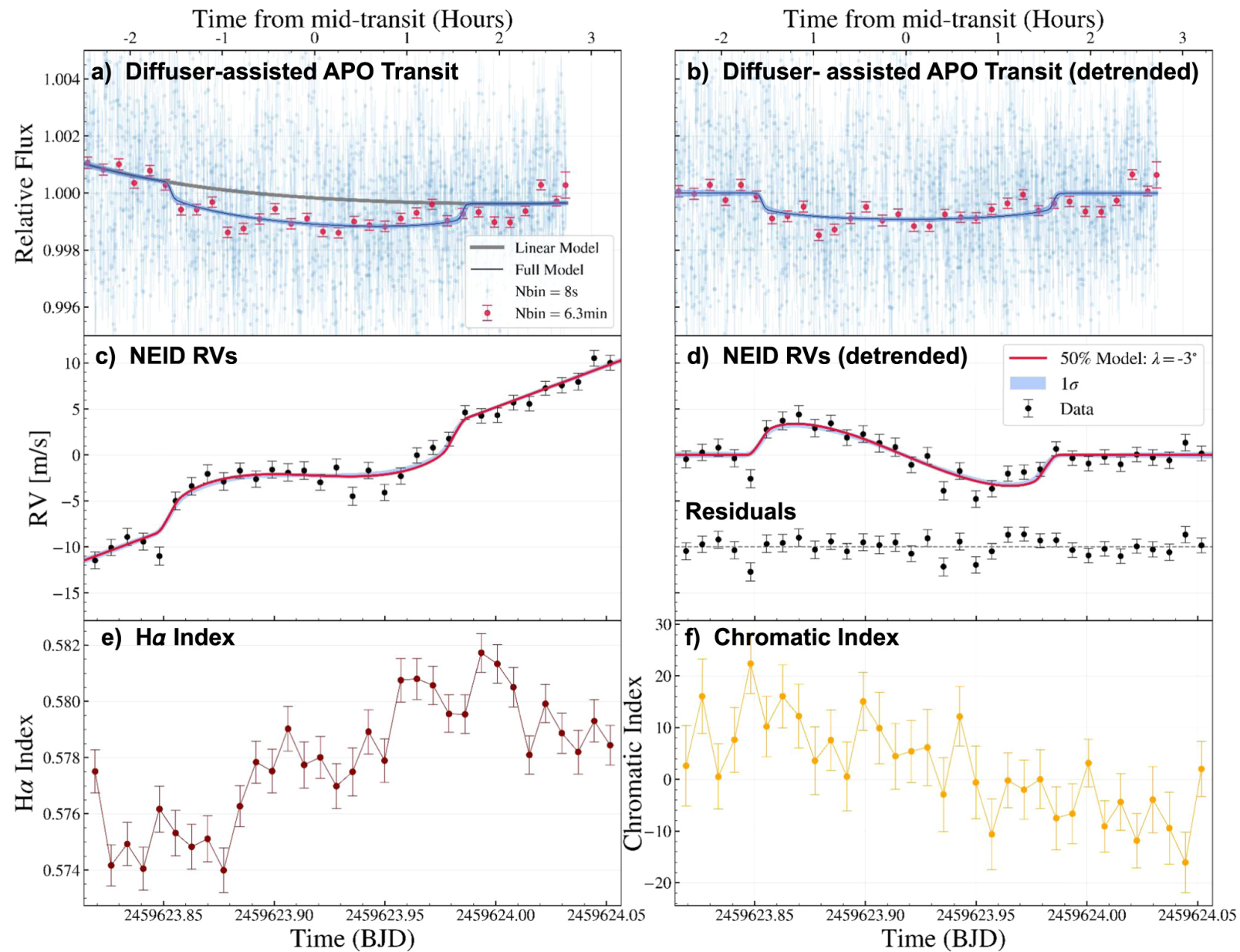
Figure 2. from Robert C. Frazier et al 2023 Astrophys. J. Lett. 944 doi:10.3847/2041-8213/acba18 https://dx.doi.org/10.3847/2041-8213/acba18 © 2023. The Author(s). Published by the American Astronomical Society.
