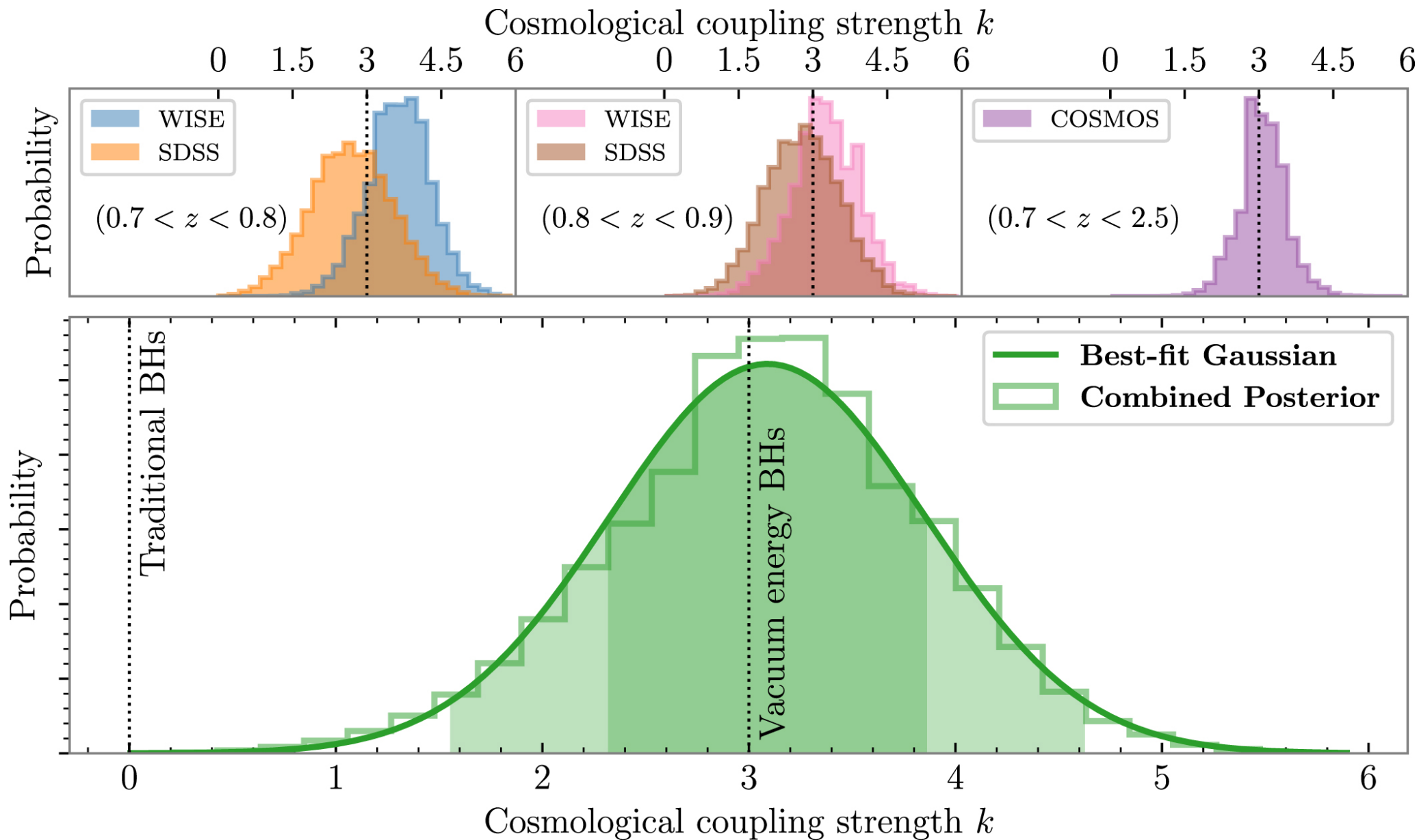
Figure 1. from Duncan Farrah et al 2023 Astrophys. J. Lett. 944 doi:10.3847/2041-8213/acb704 https://dx.doi.org/10.3847/2041-8213/acb704 © 2023. The Author(s). Published by the American Astronomical Society.
