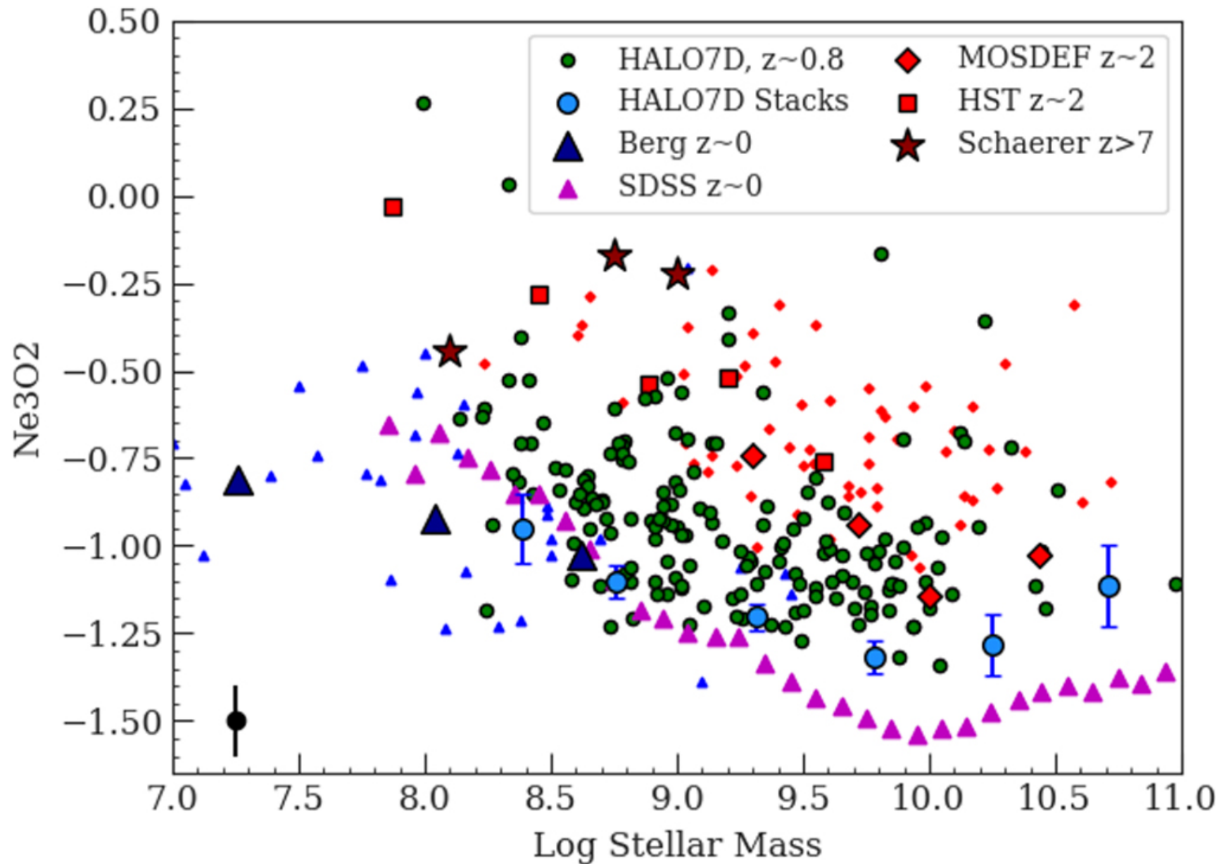
Figure 3. from John Pharo et al 2023 Astrophys. J. Lett. 946 doi:10.3847/2041-8213/acb34d https://dx.doi.org/10.3847/2041-8213/acb34d © 2023. The Author(s). Published by the American Astronomical Society.
