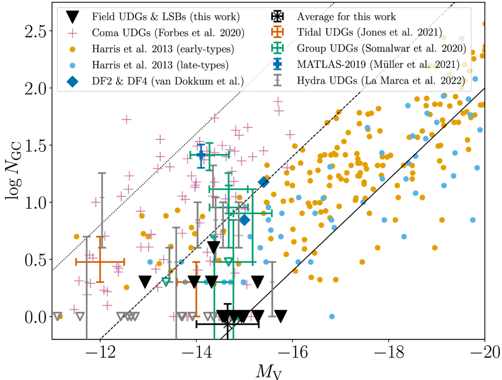
Figure 3. from Michael G. Jones et al 2023 Astrophys. J. Lett. 942 doi:10.3847/2041-8213/acaab https://dx.doi.org/10.3847/2041-8213/acaab © 2022. The Author(s). Published by the American Astronomical Society.
