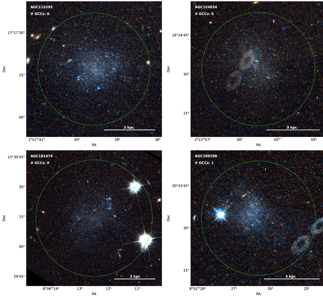
Figure 2. from Michael G. Jones et al 2023 Astrophys. J. Lett. 942 doi:10.3847/2041-8213/acaab https://dx.doi.org/10.3847/2041-8213/acaab © 2022. The Author(s). Published by the American Astronomical Society.
