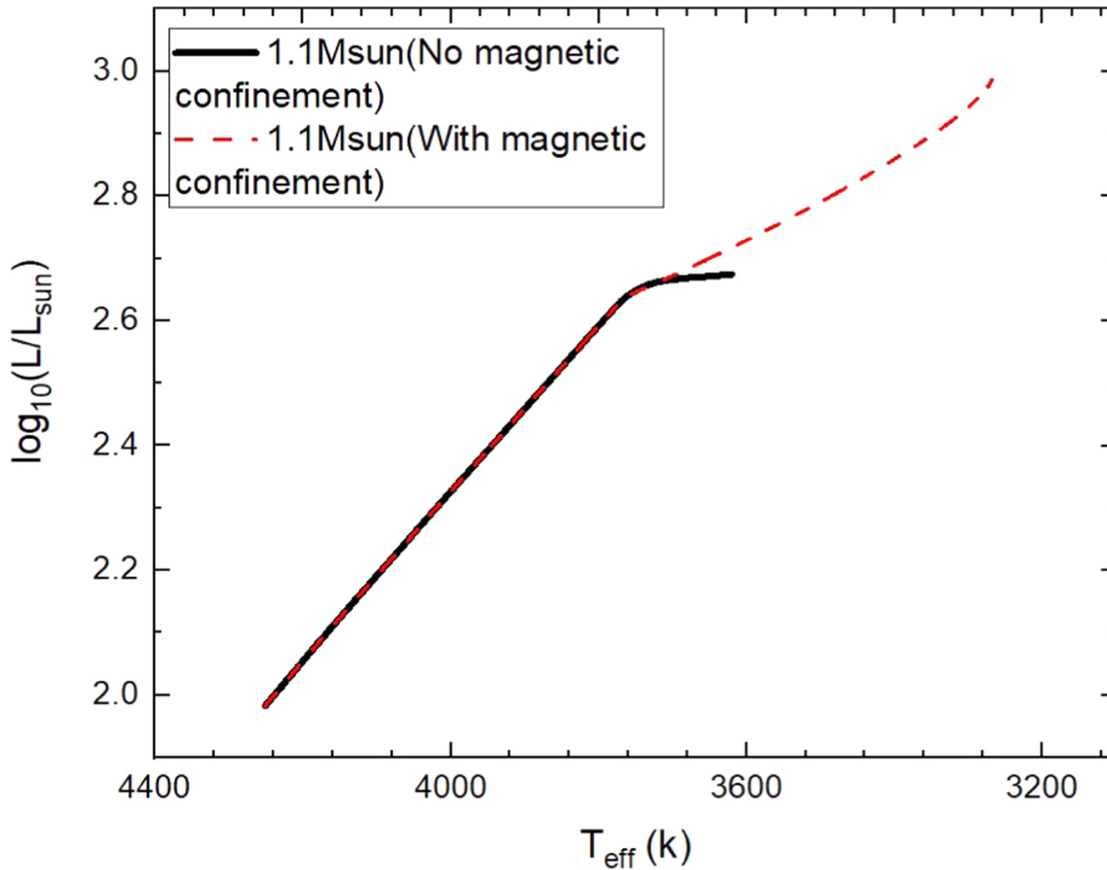
Figure 5. from Iminhaji Ablimit et al 2022 Astrophys. J. Lett. 941 doi:10.3847/2041-8213/aca806 https://dx.doi.org/10.3847/2041-8213/aca806 © 2022. The Author(s). Published by the American Astronomical Society.
