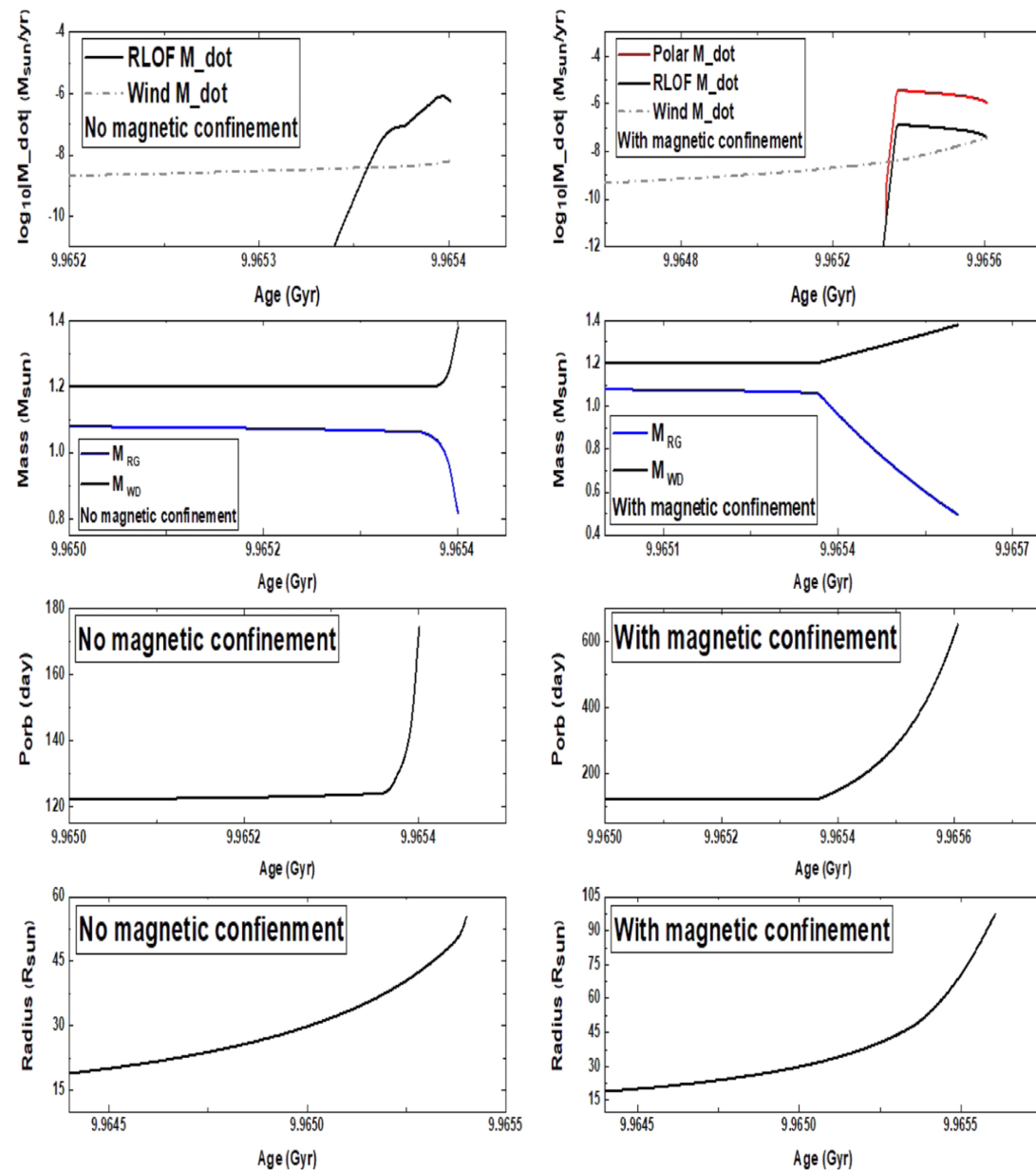
Figure 4. from Iminhaji Ablimit et al 2022 Astrophys. J. Lett. 941 doi:10.3847/2041-8213/aca806 https://dx.doi.org/10.3847/2041-8213/aca806 © 2022. The Author(s). Published by the American Astronomical Society.
