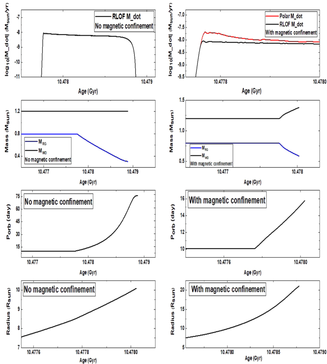
Figure 3. from Iminhaji Ablimit et al 2022 Astrophys. J. Lett. 941 doi:10.3847/2041-8213/aca806 https://dx.doi.org/10.3847/2041-8213/aca806 © 2022. The Author(s). Published by the American Astronomical Society.
