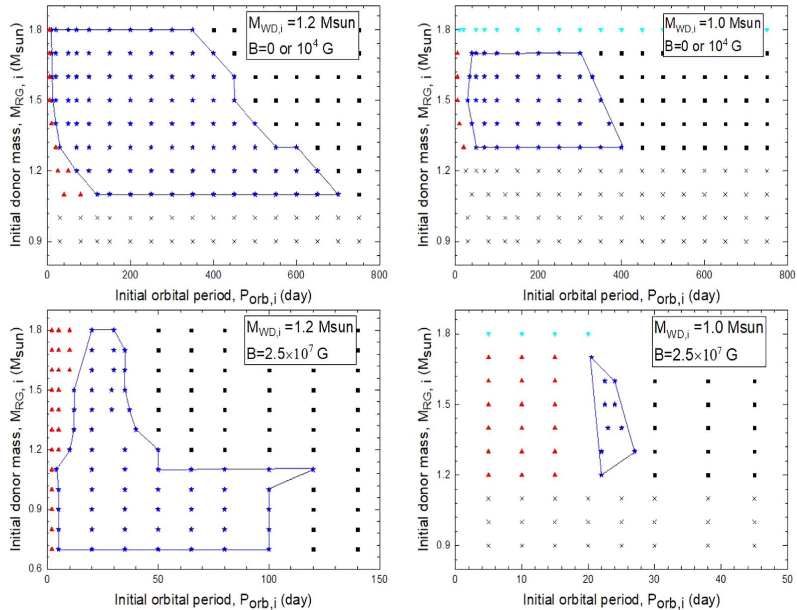
Figure 2. from Iminhaji Ablimit et al 2022 Astrophys. J. Lett. 941 doi:10.3847/2041-8213/aca806 https://dx.doi.org/10.3847/2041-8213/aca806 © 2022. The Author(s). Published by the American Astronomical Society.
