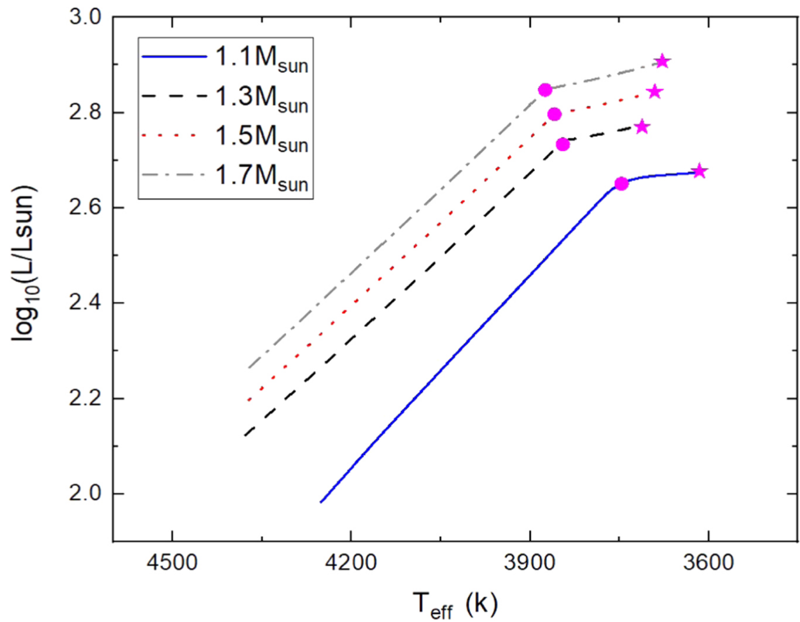
Figure 1. from Iminhaji Ablimit et al 2022 Astrophys. J. Lett. 941 doi:10.3847/2041-8213/aca806 https://dx.doi.org/10.3847/2041-8213/aca806 © 2022. The Author(s). Published by the American Astronomical Society.
