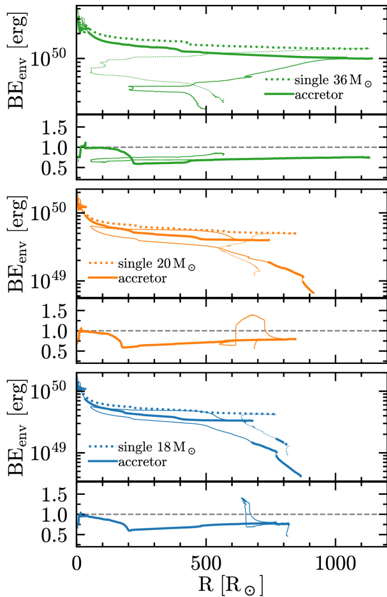
Figure 4. from M. Renzo et al 2023 Astrophys. J. Lett. 942 doi:10.3847/2041-8213/aca4d3 https://dx.doi.org/10.3847/2041-8213/aca4d3 © 2023. The Author(s). Published by the American Astronomical Society.
