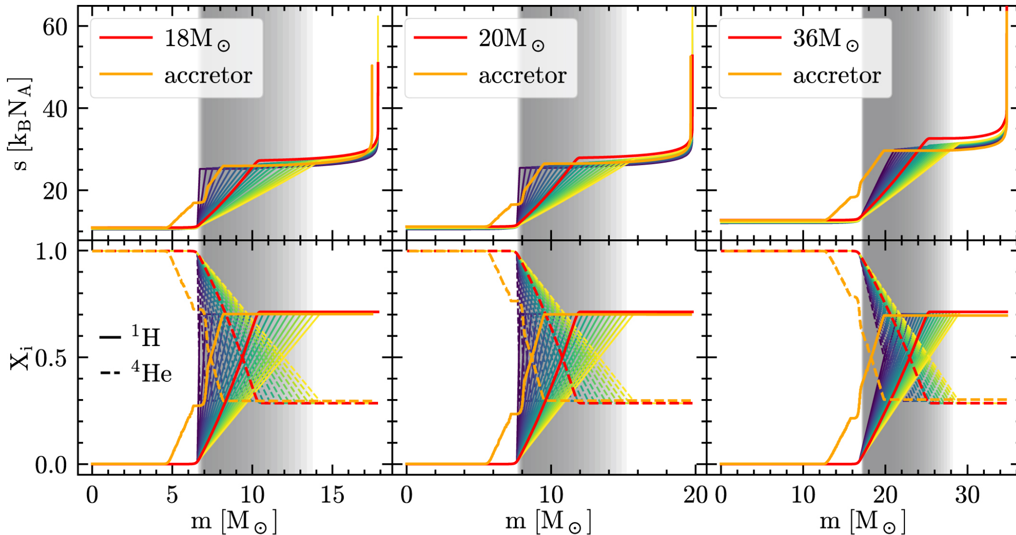
Figure 2. from M. Renzo et al 2023 Astrophys. J. Lett. 942 doi:10.3847/2041-8213/aca4d3 https://dx.doi.org/10.3847/2041-8213/aca4d3 © 2023. The Author(s). Published by the American Astronomical Society.
