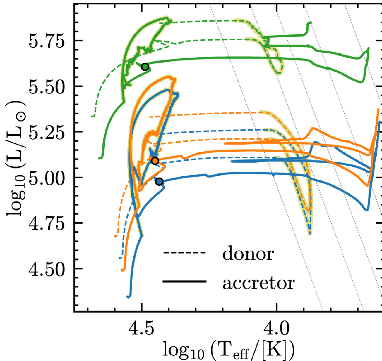
Figure 1. from M. Renzo et al 2023 Astrophys. J. Lett. 942 doi:10.3847/2041-8213/aca4d3 https://dx.doi.org/10.3847/2041-8213/aca4d3 © 2023. The Author(s). Published by the American Astronomical Society.
