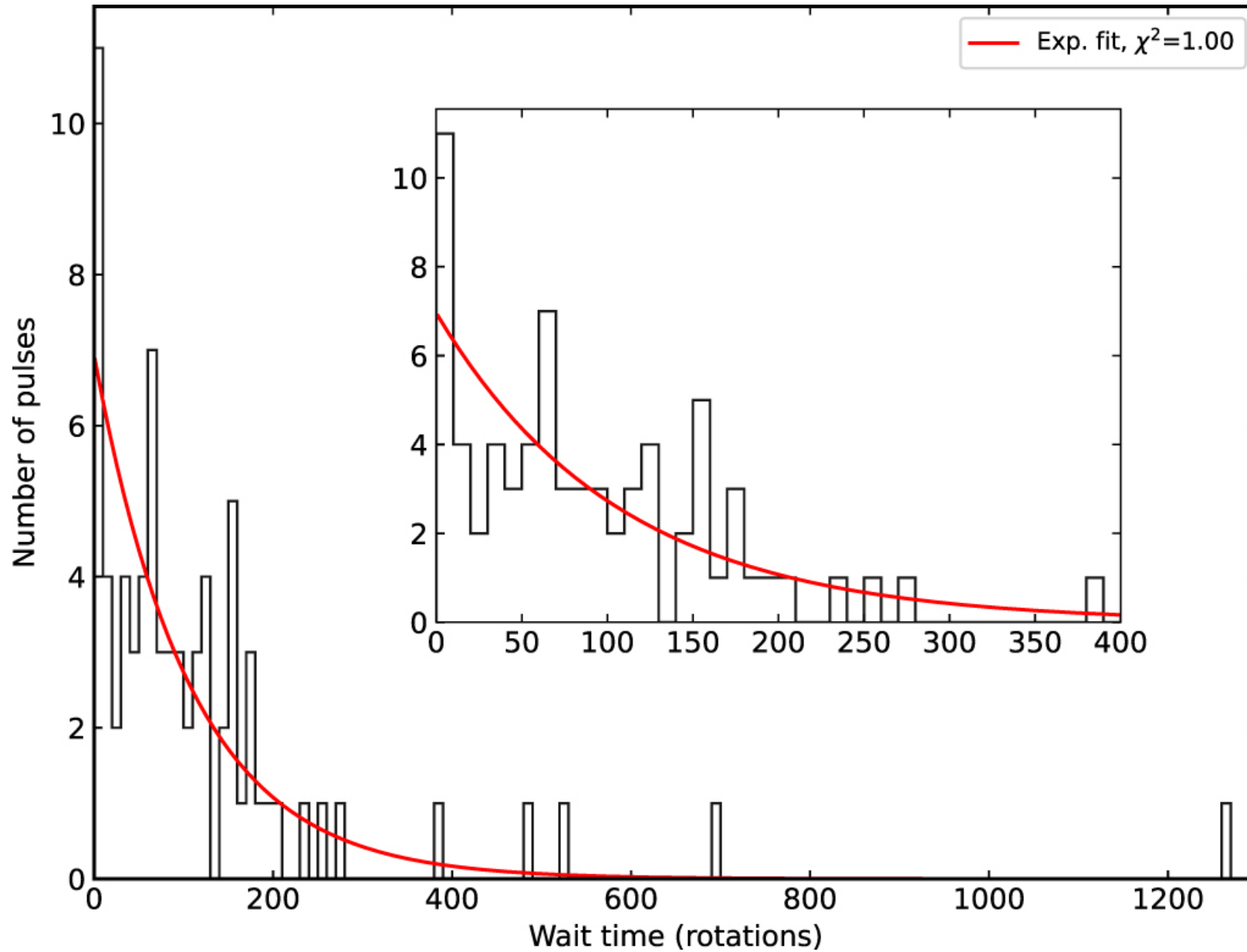
Figure 8. from Jintao Xie et al 2022 Astrophys. J. Lett. 940 doi:10.3847/2041-8213/ac9f37 https://dx.doi.org/10.3847/2041-8213/ac9f37 © 2022. The Author(s). Published by the American Astronomical Society.
