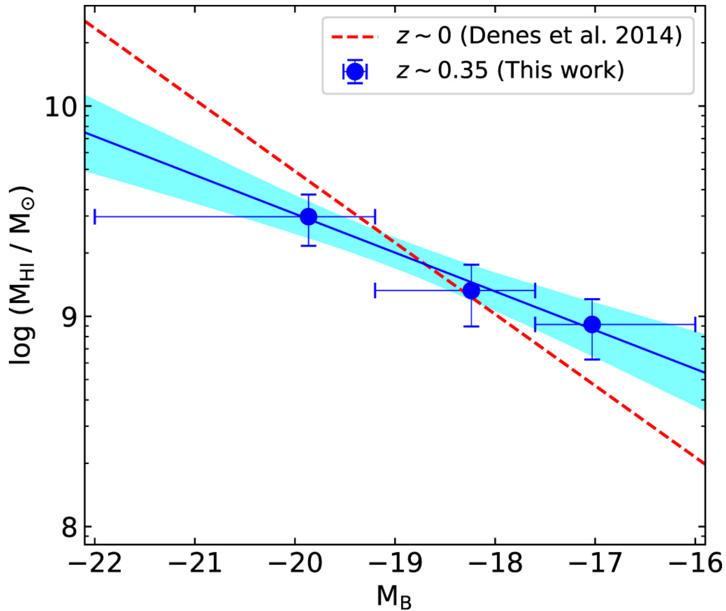
Figure 2. from Apurba Bera et al 2022 Astrophys. J. Lett. 940 doi:10.3847/2041-8213/ac9d32 https://dx.doi.org/10.3847/2041-8213/ac9d32 © 2022. The Author(s). Published by the American Astronomical Society.
