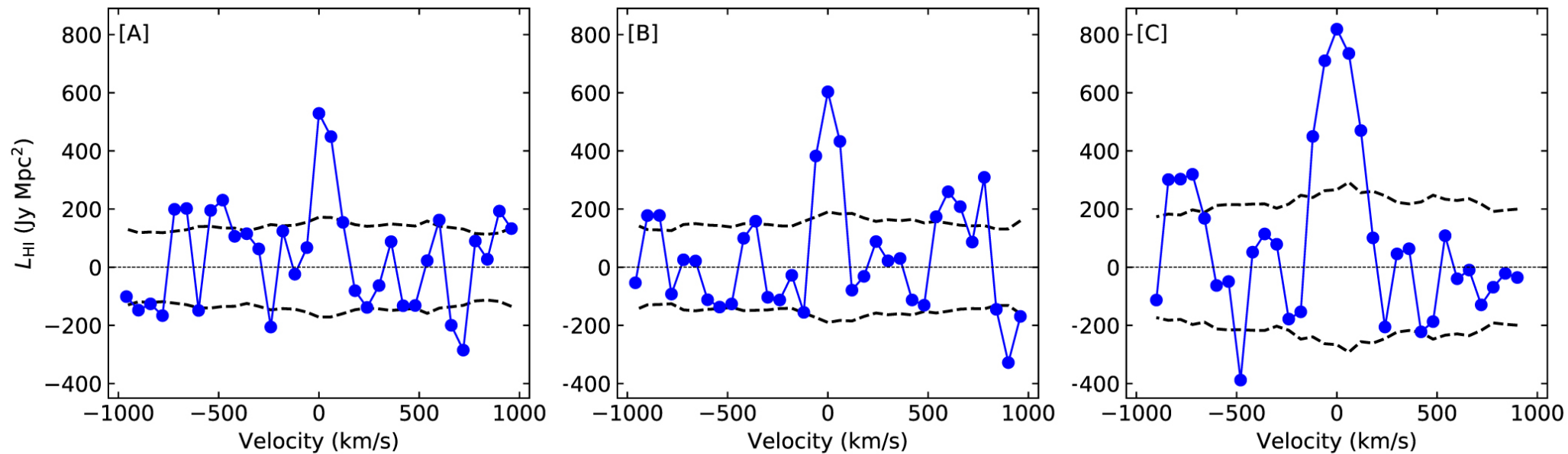
Figure 1. from Apurba Bera et al 2022 Astrophys. J. Lett. 940 doi:10.3847/2041-8213/ac9d32 https://dx.doi.org/10.3847/2041-8213/ac9d32 © 2022. The Author(s). Published by the American Astronomical Society.
