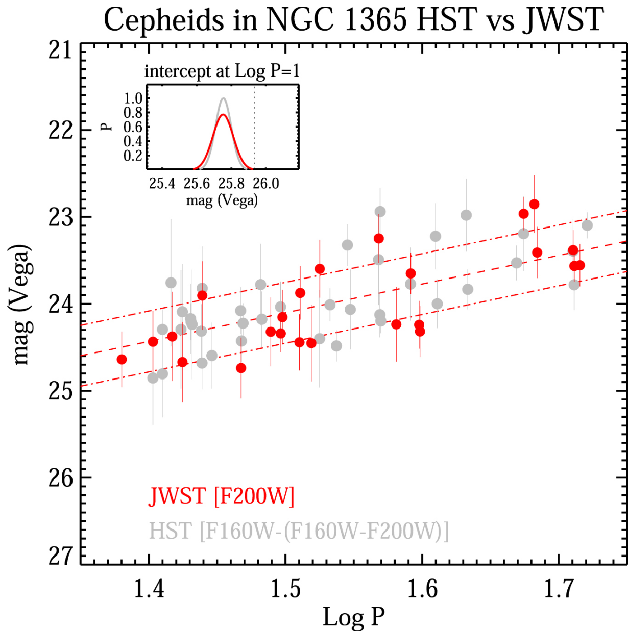
Figure 3. from Wenlong Yuan et al 2022 Astrophys. J. Lett. 940 doi:10.3847/2041-8213/ac9b27 https://dx.doi.org/10.3847/2041-8213/ac9b27 © 2022. The Author(s). Published by the American Astronomical Society.
