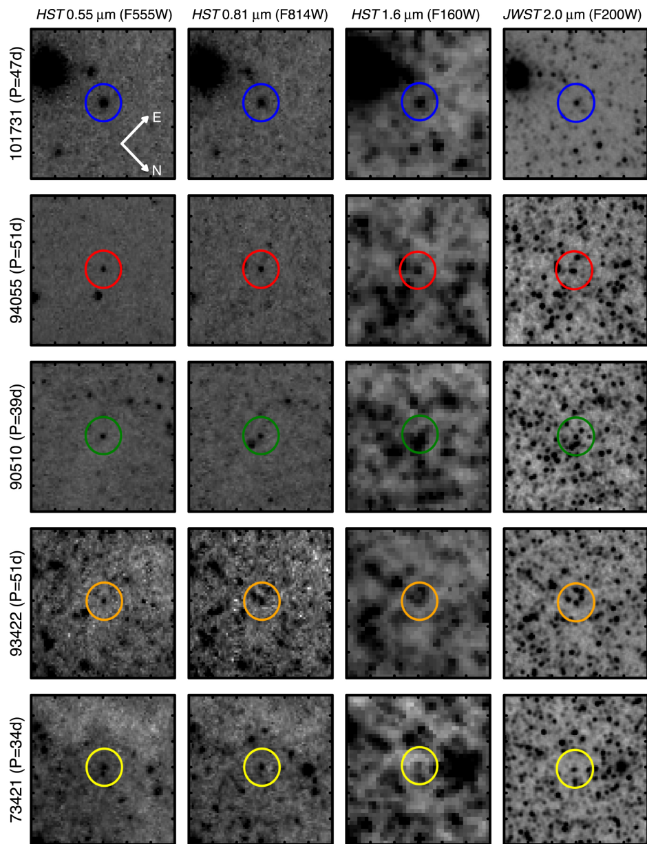
Figure 2. from Wenlong Yuan et al 2022 Astrophys. J. Lett. 940 doi:10.3847/2041-8213/ac9b27 https://dx.doi.org/10.3847/2041-8213/ac9b27 © 2022. The Author(s). Published by the American Astronomical Society.
