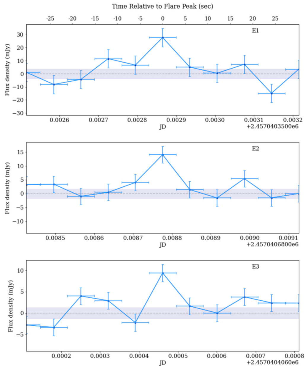
Figure 2. from Kiana Burton et al 2022 Astrophys. J. Lett. 939 doi:10.3847/2041-8213/ac9973 https://dx.doi.org/10.3847/2041-8213/ac9973 © 2022. The Author(s). Published by the American Astronomical Society.
