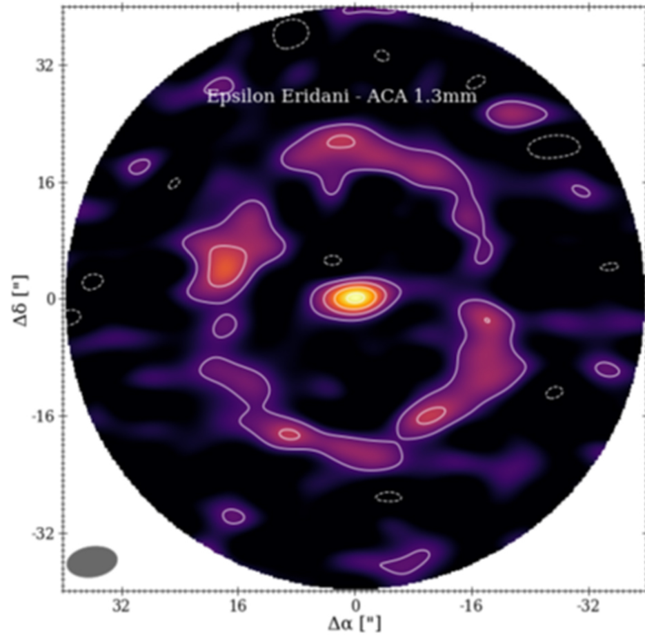
Figure 1. from Kiana Burton et al 2022 Astrophys. J. Lett. 939 doi:10.3847/2041-8213/ac9973 https://dx.doi.org/10.3847/2041-8213/ac9973 © 2022. The Author(s). Published by the American Astronomical Society.
