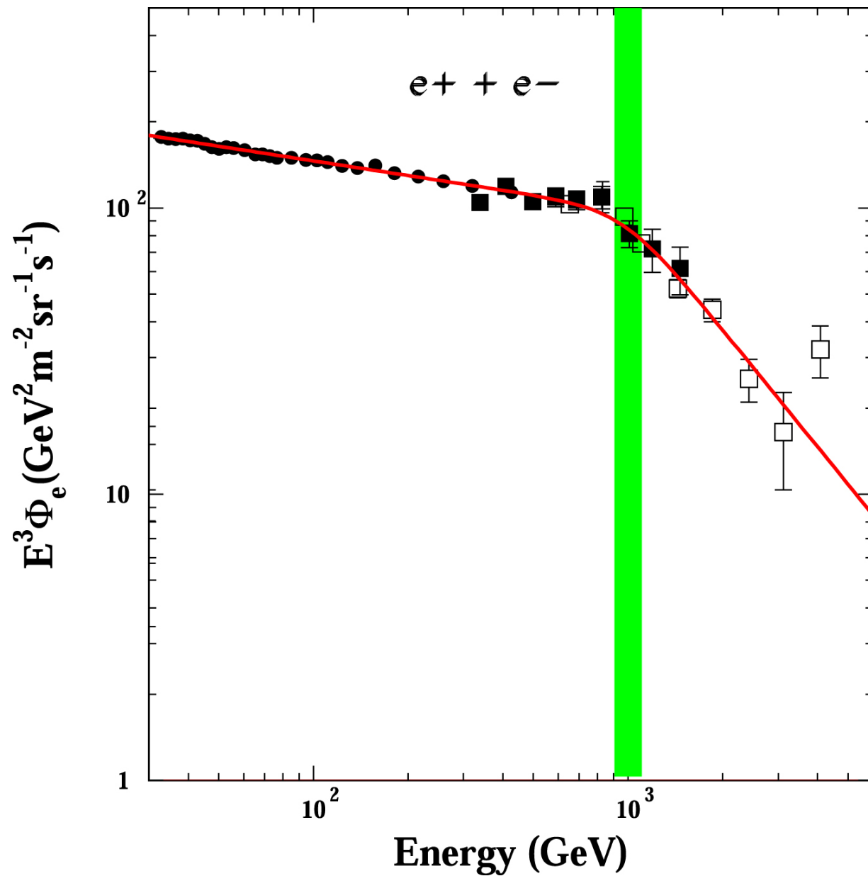
Figure 1. from Shlomo Dado and Arnon Dar 2022 Astrophys. J. Lett. 940 doi:10.3847/2041-8213/ac98c8 https://dx.doi.org/10.3847/2041-8213/ac98c8 © 2022. The Author(s). Published by the American Astronomical Society.
