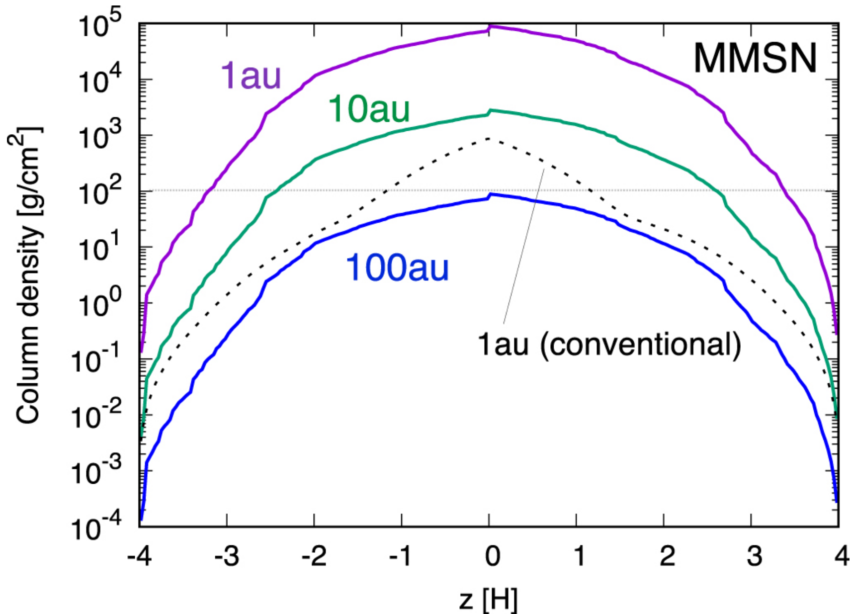
Figure 6. from Yuri I. Fujii and Shigeo S. Kimura 2022 Astrophys. J. Lett. 937 doi:10.3847/2041-8213/ac86c2 https://dx.doi.org/10.3847/2041-8213/ac86c2 © 2022. The Author(s). Published by the American Astronomical Society.
