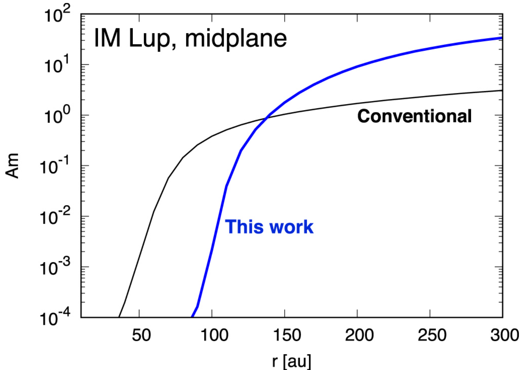
Figure 5. from Yuri I. Fujii and Shigeo S. Kimura 2022 Astrophys. J. Lett. 937 doi:10.3847/2041-8213/ac86c2 https://dx.doi.org/10.3847/2041-8213/ac86c2 © 2022. The Author(s). Published by the American Astronomical Society.
