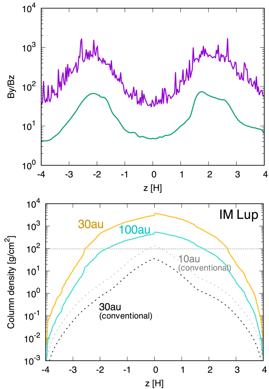
Figure 2. from Yuri I. Fujii and Shigeo S. Kimura 2022 Astrophys. J. Lett. 937 doi:10.3847/2041-8213/ac86c2 https://dx.doi.org/10.3847/2041-8213/ac86c2 © 2022. The Author(s). Published by the American Astronomical Society.
