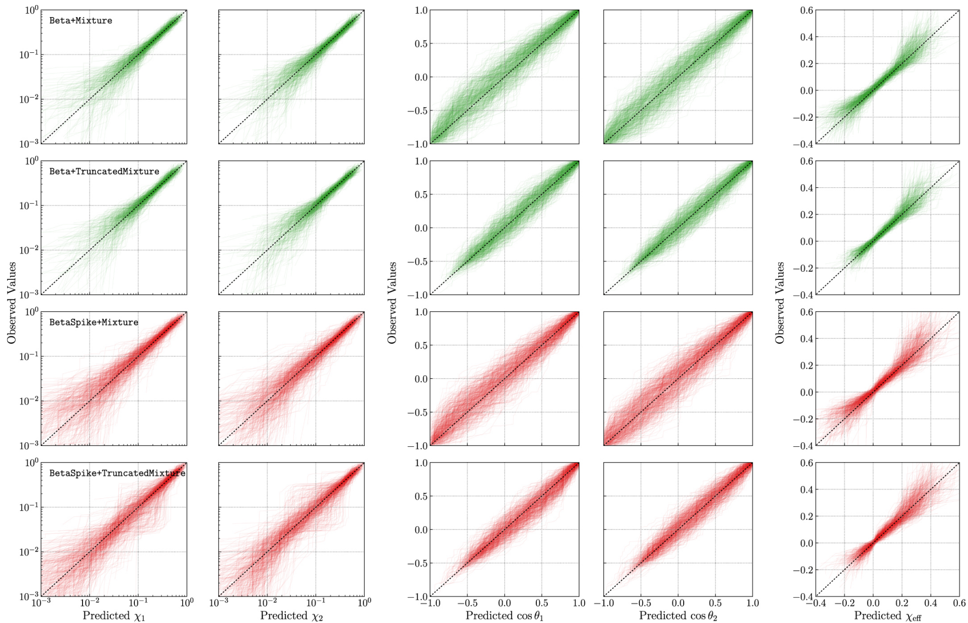
Figure 9. from Thomas A. Callister et al 2022 Astrophys. J. Lett. 937 doi:10.3847/2041-8213/ac847e https://dx.doi.org/10.3847/2041-8213/ac847e © 2022. The Author(s). Published by the American Astronomical Society.
